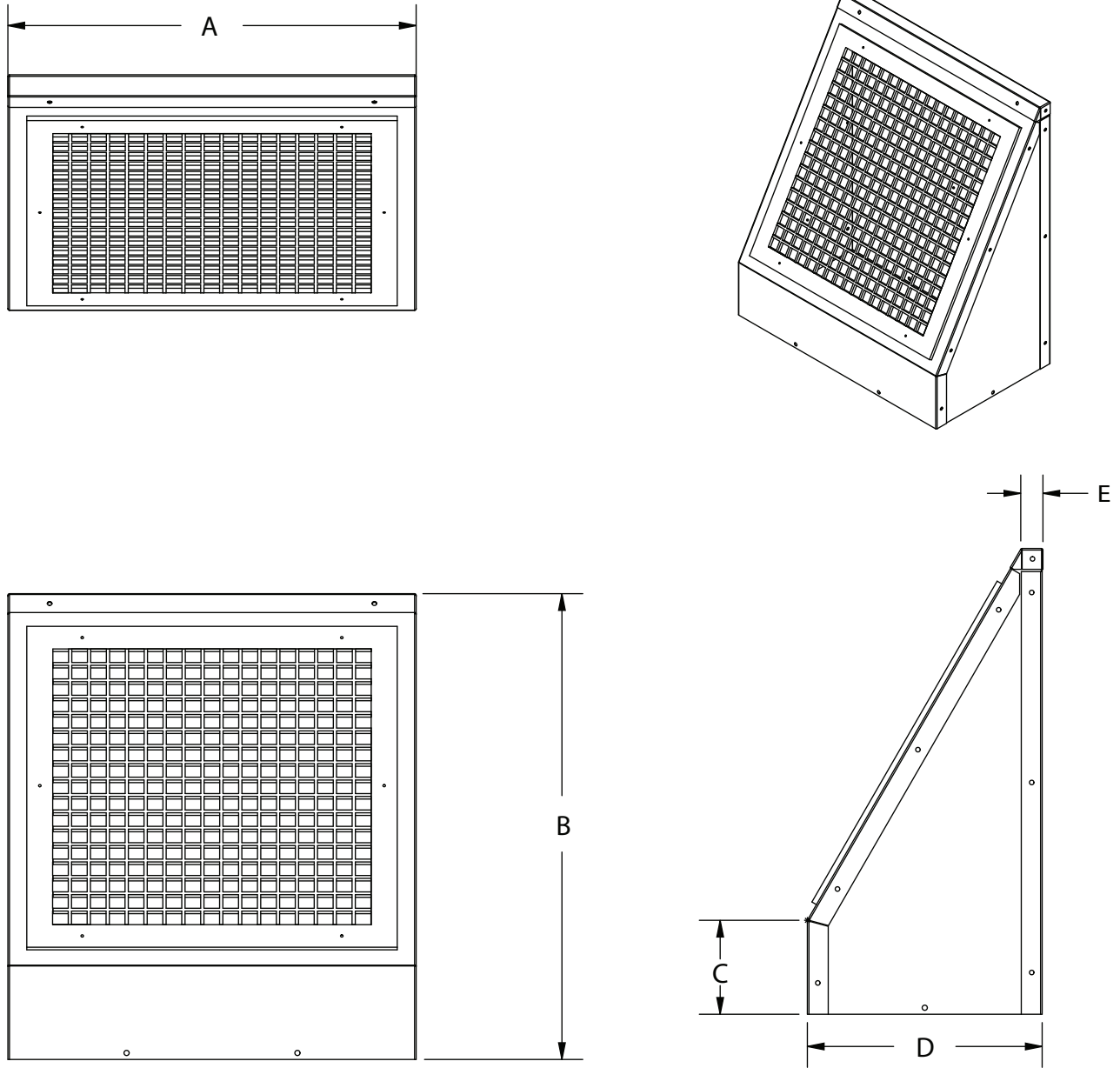
Fig. 1 – Dimensions (KFADG0101LRG shown)
